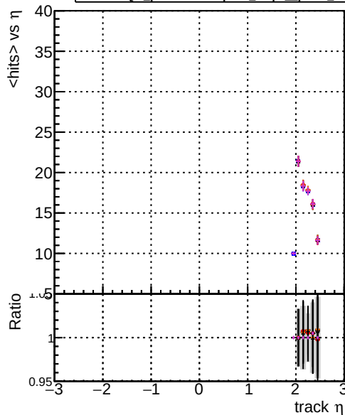
DOM original step2_pt200_eta2p0to2p5 DOM mkFit_step2_pt200_eta2p0to2p5 DOM angle_step2_pt200_eta2p0to2p5 DOM fast_step2_pt200_eta2p0to2p5 DOM pixelCPEtemplate_step2_pt200_eta2p0to2p5 mean hits
