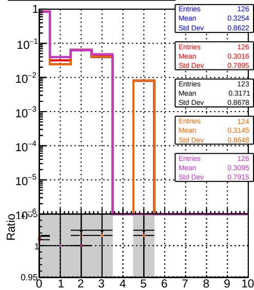
DOM original step2_pt200_eta2p0to2p5 DOM mkFit_step2_pt200_eta2p0to2p5 DOM angle_step2_pt200_eta2p0to2p5 DOM fast_step2_pt200_eta2p0to2p5 DOM pixelCPEtemplate_step2_pt200_eta2p0to2p5 mean hits
