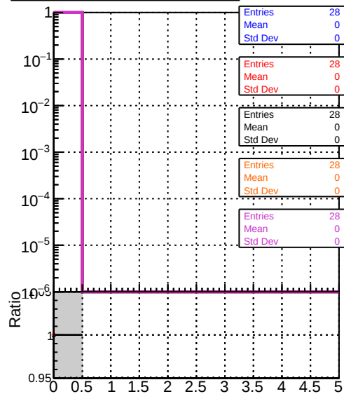
DOM original step2_pt1to20_eta2p5to4p0 DOM mkrFit_step2_pt1to20_eta2p5to4p0 DOM angle_step2_pt1to20_eta2p5to4p0 DOM fast_step2_pt1to20_eta2p5to4p0 DOM pixelCPEtemplate_step2_pt1to20_eta2p5to4p0 mean hits
