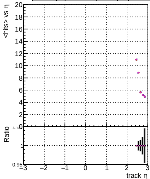
mean hits vs \eta DOM original step2_pt1to20_eta2p5to4p0 DOM mkrFit_step2_pt1to20_eta2p5to4p0 DOM angle_step2_pt1to20_eta2p5to4p0 DOM fast_step2_pt1to20_eta2p5to4p0 DOM pixelCPEtemplate_step2_pt1to20_eta2p5to4p0
