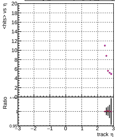
DOM original step2_pt1to20_eta2p5to4p0 DOM mkrFit_step2_pt1to20_eta2p5to4p0 DOM angle_step2_pt1to20_eta2p5to4p0 DOM fast_step2_pt1to20_eta2p5to4p0 DOM pixelCPEtemplate_step2_pt1to20_eta2p5to4p0
