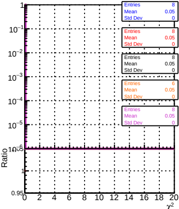
normalized \chi^2
