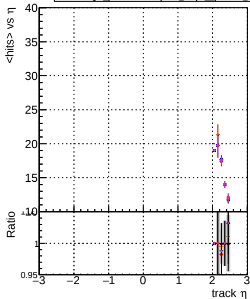
DOM original_step2_pt1to20_eta2p0to2p5 DOM mkrfit_step2_pt1to20_eta2p0to2p5 DOM angle_step2_pt1to20_eta2p0to2p5 DOM fast_step2_pt1to20_eta2p0to2p5 DOM pixelCPEtemplate_step2_pt1to20_eta2p0to2p5
