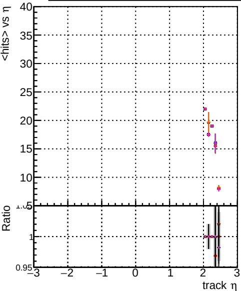
mean hit DOM original_step2_pt1to20_eta2p0to2p5 DOM mkrFit_step2_pt1to20_eta2p0to2p5 DOM angle_step2_pt1to20_eta2p0to2p5 DOM fast_step2_pt1to20_eta2p0to2p5 DOM pixelCPEtemplate_step2_pt1to20_eta2p0to2p5
