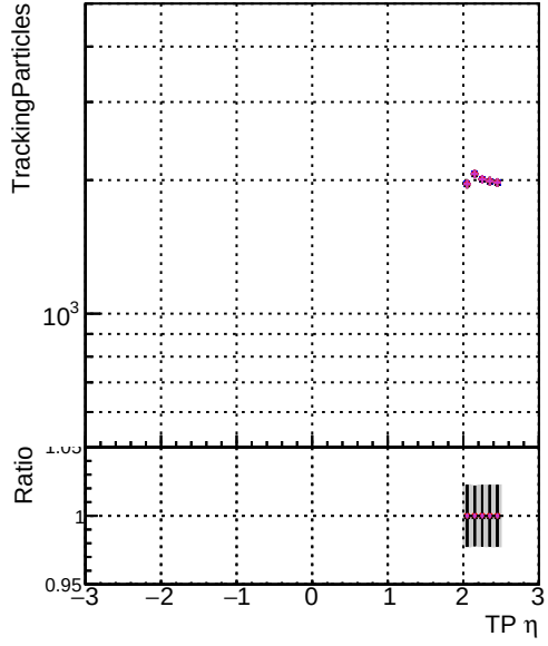
—•— DOM original_step2_pt1to20_eta2p0to2p5 —•— DOM mkFit_step2_pt1to20_eta2p0to2p5 —•— DOM angle_step2_pt1to20_eta2p0to2p5 —•— DOM fast_step2_pt1to20_eta2p0to2p5 —•— DOM pixelCPEtemplate_step2_pt1to20_eta2p0to2p5
