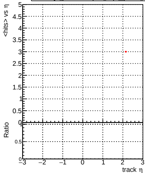
DOM original step2_pt1to20_eta2p0to2p5 DOM mkrFit_step2_pt1to20_eta2p0to2p5 DOM angle_step2_pt1to20_eta2p0to2p5 DOM fast_step2_pt1to20_eta2p0to2p5 DOM_pixelCPEtemplate_step2_pt1to20_eta2p0to2p5 mean hit
