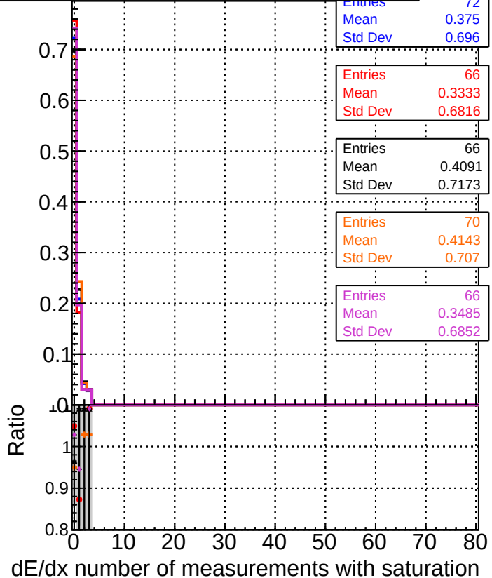
DQM original step2 pt1to20 eta2p0to2p5 DQM mkFit step2 pt1to20 eta2p0to2p5 DQM angle step2 pt1to20 eta2p0to2p5 DQM fast step2 pt1to20 eta2p0to2p5 DQM pixelCPE template step2 pt1to20 eta2p0to2p5
