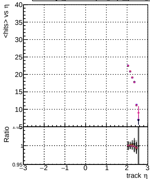
mean hit DOM original step2_pt1to20_eta2p0to2p5 DOM mkFit_step2_pt1to20_eta2p0to2p5 DOM angle_step2_pt1to20_eta2p0to2p5 DOM fast_step2_pt1to20_eta2p0to2p5 DOM pixelCPEtemplate_step2_pt1to20_eta2p0to2p5
