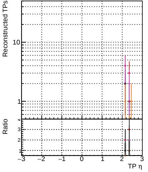
— DQM original_step2_pt1to20_eta2p0to2p5 — DQM mkFit_step2_pt1to20_eta2p0to2p5 — DQM angle_step2_pt1to20_eta2p0to2p5 — DQM fast_step2_pt1to20_eta2p0to2p5 — DQM pixelCPEtemplate_step2_pt1to20_eta2p0to2p5
