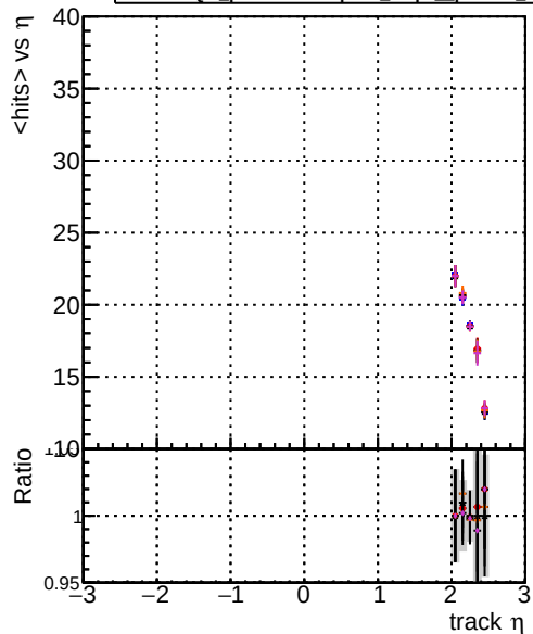
DOM original step2_pt1to20_eta2p0to2p5 DOM mkFit_step2_pt1to20_eta2p0to2p5 DOM angle_step2_pt1to20_eta2p0to2p5 DOM fast_step2_pt1to20_eta2p0to2p5 DOM pixelCPEtemplate_step2_pt1to20_eta2p0to2p5
