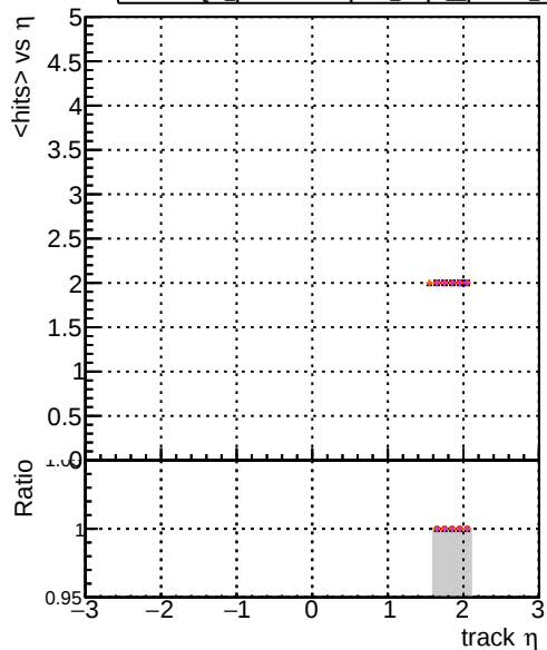
DOM original_step2_pt1to20_eta1p6to2p0 DOM mkrFit_step2_pt1to20_eta1p6to2p0 DOM angle_step2_pt1to20_eta1p6to2p0 DOM fast_step2_pt1to20_eta1p6to2p0 DOM pixelCPEtemplate_step2_pt1to20_eta1p6to2p0
