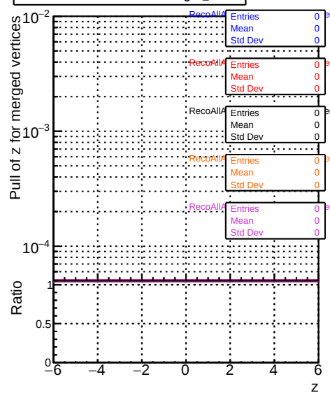
RecoAllAssoc2GenMatchedMerged_PullZ
