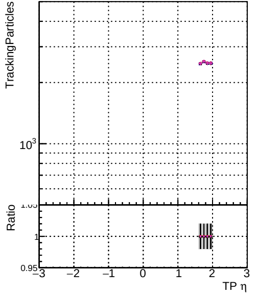
—•— DQM original_step2_pt1to20_eta1p6to2p0 —•— DQM mkFit_step2_pt1to20_eta1p6to2p0 —•— DQM angle_step2_pt1to20_eta1p6to2p0 —•— DQM fast_step2_pt1to20_eta1p6to2p0 —•— DQM pixelCPEtemplate_step2_pt1to20_eta1p6to2p0
