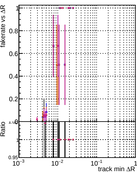
Fake rate vs \Delta R(\text{track, jet}) DOM original_step2 pt1to20_eta1p4to1p6 angle_step2 pt1to20_eta1p4to1p6 fixedCP-Template_step2 pt1to20_eta1p4to1p6
