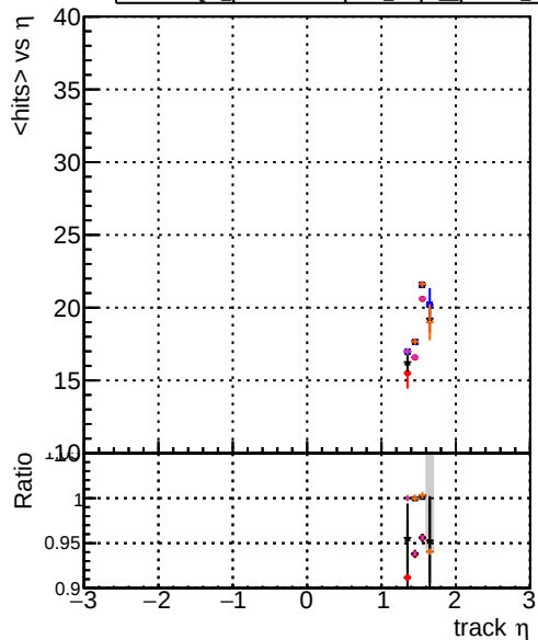
mean hits vs \eta DOM original step2_pt1to20_eta1p4to1p6 DOM mkFit step2_pt1to20_eta1p4to1p6 DOM angle step2_pt1to20_eta1p4to1p6 DOM fast step2_pt1to20_eta1p4to1p6 DOM pixelCPEtemplate_step2_pt1to20_eta1p4to1p6
