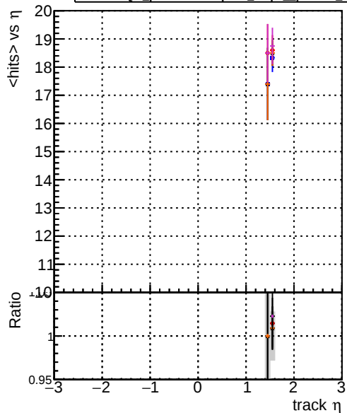
mean hit DOM original step2 pt1to20 eta1p4to1p6 DOM mkFit step2 pt1to20 eta1p4to1p6 DOM angle step2 pt1to20 eta1p4to1p6 DOM fast step2 pt1to20 eta1p4to1p6 DOM pixelCPE template step2 pt1to20 eta1p4to1p6
