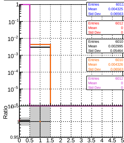
mean hits vs \eta DOM original step2_pt1to20_eta1p4to1p6 DOM mkrfit_step2_pt1to20_eta1p4to1p6 DOM angle_step2_pt1to20_eta1p4to1p6 DOM fast_step2_pt1to20_eta1p4to1p6 DOM pixelCPEtemplate_step2_pt1to20_eta1p4to1p6
