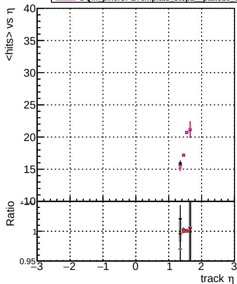
mean hits vs \eta DOM original step2_pt1to20_eta1p4to1p6 DOM mkrfit_step2_pt1to20_eta1p4to1p6 DOM angle_step2_pt1to20_eta1p4to1p6 DOM fast_step2_pt1to20_eta1p4to1p6 DOM pixelCPEtemplate_step2_pt1to20_eta1p4to1p6
