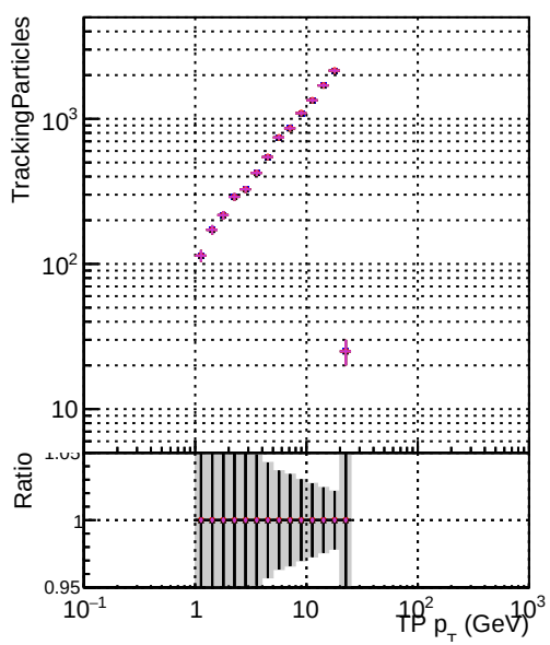
—•— DOM original_step2_pt1to20_eta1p4to1p6 —•— DOM mkFit_step2_pt1to20_eta1p4to1p6 —•— DOM angle_step2_pt1to20_eta1p4to1p6 —•— DOM fast_step2_pt1to20_eta1p4to1p6 —•— DOM pixelCPEtemplate_step2_pt1to20_eta1p4to1p6
