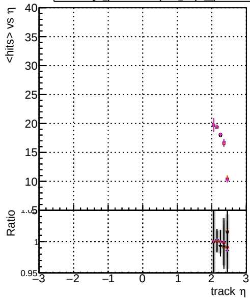
DOM original step2_pt10to1000_eta2p0to2p5 DOM mkrfit_step2_pt10to1000_eta2p0to2p5 DOM angle_step2_pt10to1000_eta2p0to2p5 DOM fast_step2_pt10to1000_eta2p0to2p5 DOM pixelCPEtemplate_step2_pt10to1000_eta2p0to2p5
