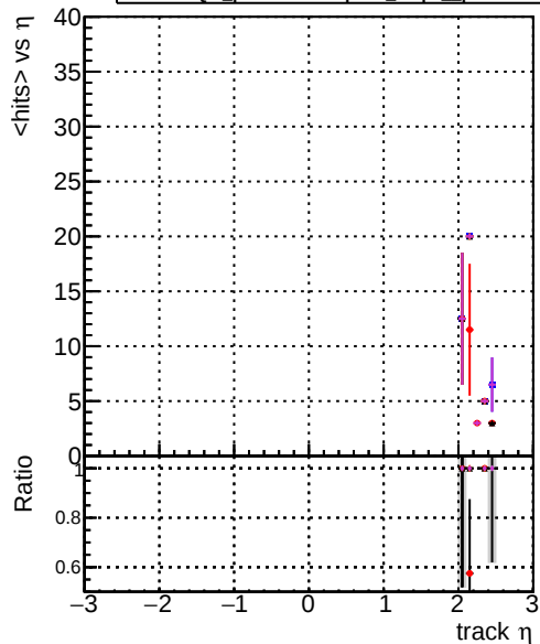
DOM original_step2_pt1to1000_eta2p0to2p5 DOM mkrfit_step2_pt1to1000_eta2p0to2p5 DOM angle_step2_pt1to1000_eta2p0to2p5 DOM fast_step2_pt1to1000_eta2p0to2p5 DOM pixelCPEtemplate_step2_pt1to1000_eta2p0to2p5
