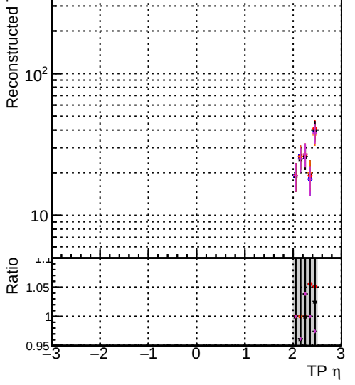
N of associated tracks (simToReco) vs eta
