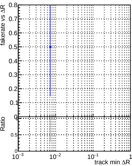
Fake rate vs \Delta R(\text{track}, \text{jet}) DQM original step2 pt1to1000 eta2p0to2p5 DQM angle step2 pt1to1000 eta2p0to2p5 DQM angle step2 pt1to1000 eta2p0to2p5 DQM pixelCPE template step2 pt1to1000 eta2p0to2p5
