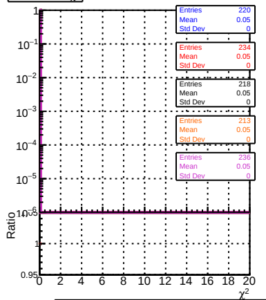
normalized \chi^2
