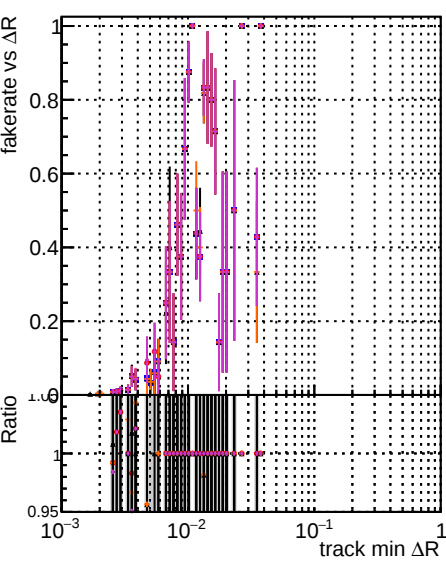
Fake rate vs \Delta R(\text{track, jet}) DOM original_step2 pt1to1000_eta1p6to2p0 angle_step2 pt1to1000_eta1p6to2p0 fixedCP-Template_step2_pt1to1000_eta1p6to2p0
