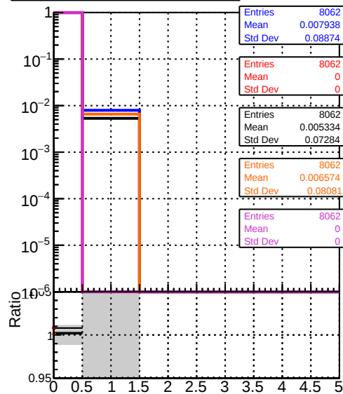
mean hits vs \eta DOM original step2_pt10to1000_eta1p6to2p0 DOM mkrFit_step2_pt10to1000_eta1p6to2p0 DOM angle_step2_pt10to1000_eta1p6to2p0 DOM fast step2_pt10to1000_eta1p6to2p0 DOM pixelCPEtemplate_step2_pt10to1000_eta1p6to2p0
