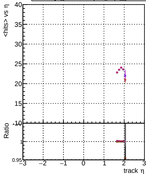
mean hits vs \eta DOM original step2_pt10to1000_eta1p6to2p0 DOM mkrFit_step2_pt10to1000_eta1p6to2p0 DOM angle_step2_pt10to1000_eta1p6to2p0 DOM fast step2_pt10to1000_eta1p6to2p0 DOM pixelCPEtemplate_step2_pt10to1000_eta1p6to2p0
