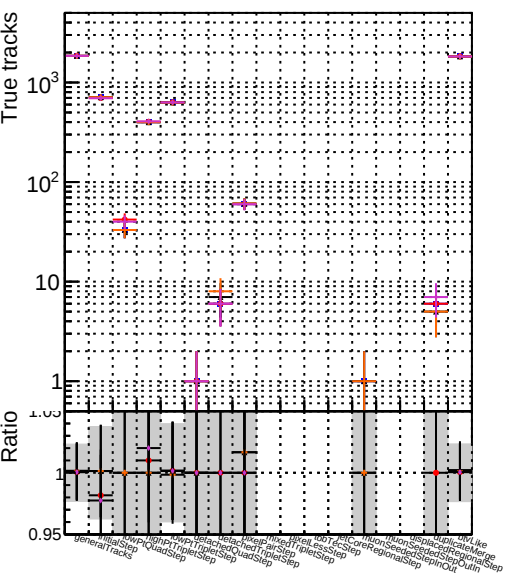
Number Legend: DOM original step2 pt1000 eta2p5to4p0 DOM mkFit step2 pt1000 eta2p5to4p0 DOM angle step2 pt1000 eta2p5to4p0 DOM fast step2 pt1000 eta2p5to4p0 DOM pixelCPEtemplate step2 pt1000 eta2p5to4p0
