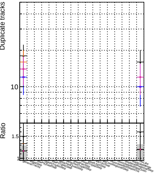
Number Legend: DOM original step2 pt1000 eta2p5to4p0 DOM mkFit step2 pt1000 eta2p5to4p0 DOM angle step2 pt1000 eta2p5to4p0 DOM fast step2 pt1000 eta2p5to4p0 DOM pixelCPEtemplate step2 pt1000 eta2p5to4p0
