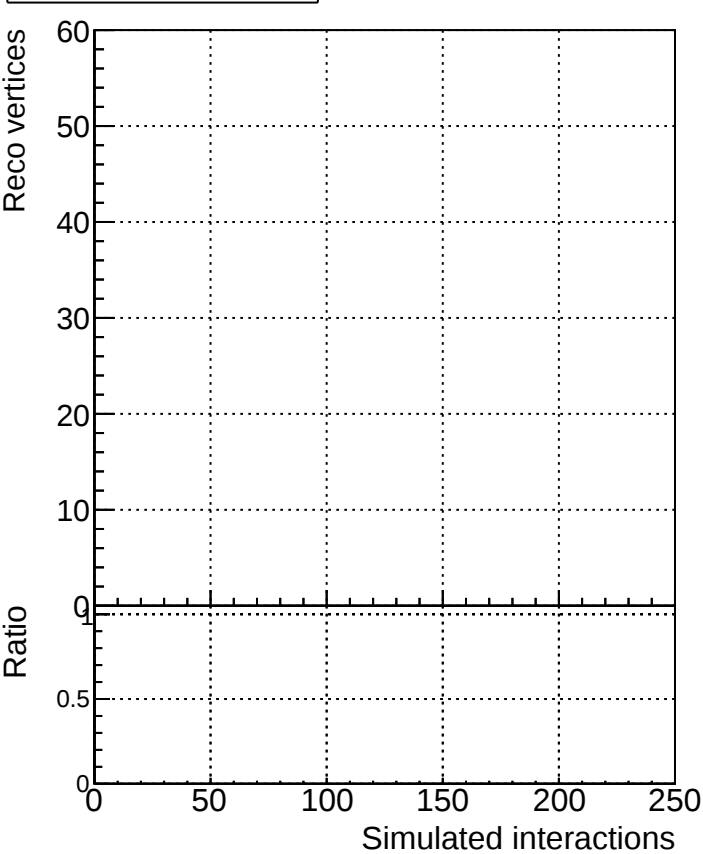
RecoVtx_vs_GenVtx
