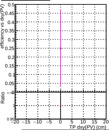
Efficiency vs Dxy(PV) (cm) DOM_original_step2_pt1000_eta2p0to2p5 DOM_mkFit_step2_pt1000_eta2p0to2p5 DOM_angle_step2_pt1000_eta2p0to2p5 DOM_fast_step2_pt1000_eta2p0to2p5 DOM_pixelCPETemplate_step2_pt1000_eta2p0to2p5
