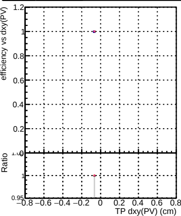
Efficiency vs Dxy(PV) (cm) DOM_original_step2_pt1000_eta2p0to2p5 DOM_mkFit_step2_pt1000_eta2p0to2p5 DOM_angle_step2_pt1000_eta2p0to2p5 DOM_fast_step2_pt1000_eta2p0to2p5 DOM_pixelCPETemplate_step2_pt1000_eta2p0to2p5
