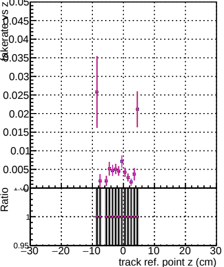
Fake rate vs v Legend: original_step2_pt1000_eta2p0to2p5 angle_step2_pt1000_eta2p0to2p5 fixerCP-Template_step2_pt1000_eta2p0to2p5
