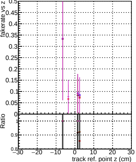
Fake rate vs v DOM original step2 pt1000 eta2p0to2p5 DOM angle step2 pt1000 eta2p0to2p5 DOM angle step2 pt1000 eta2p0to2p5 DOM pixelCP template step2 pt1000 eta2p0to2p5
