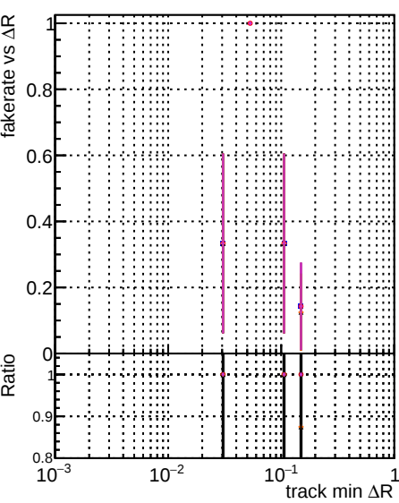
Fake rate vs ΔR(track, jet) for different methods: DOM original_step2_pt1000_eta2p0to2p5, DOM angle_step2_pt1000_eta2p0to2p5, DOM fixedCPETemplate_step2_pt1000_eta2p0to2p5
