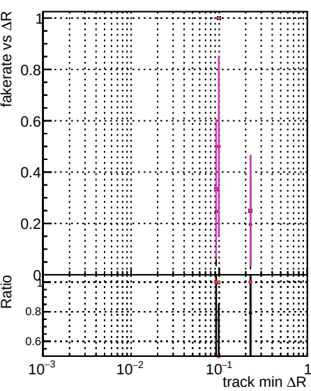
Fake rate vs \Delta R(\text{track, jet}) original step2 pt1000 eta2p0to2p5 angle step2 pt1000 eta2p0to2p5 fixed CP template step2 pt1000 eta2p0to2p5
