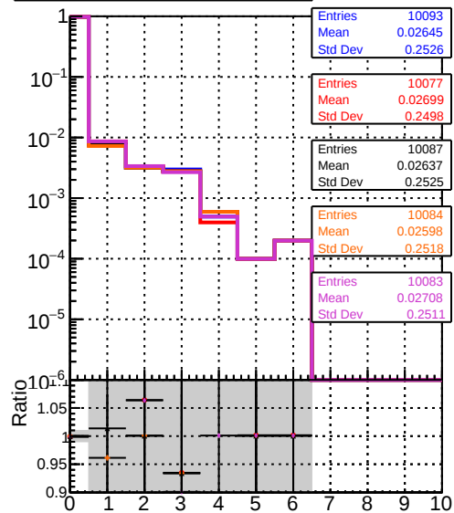
DOM original_step2_pt1000_eta2p0to2p5 DOM mkrfit_step2_pt1000_eta2p0to2p5 DOM angle_step2_pt1000_eta2p0to2p5 DOM fast_step2_pt1000_eta2p0to2p5 DOM pixelCPEtemplate_step2_pt1000_eta2p0to2p5
