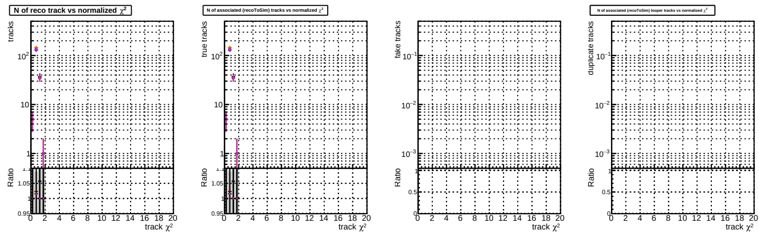
N of reco track vs. \chi^2 Legend: DOM original step2 - p1000 eta2p0to2p5 DOM prime step2 - p1000 eta2p0to2p5 DOM fixedCP template step2 - p1000 eta2p0to2p5
