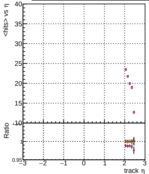
mean hit DOM original_step2_pt1000_eta2p0to2p5 DOM mkFit_step2_pt1000_eta2p0to2p5 DOM angle_step2_pt1000_eta2p0to2p5 DOM fast_step2_pt1000_eta2p0to2p5 DOM pixelCPEtemplate_step2_pt1000_eta2p0to2p5
