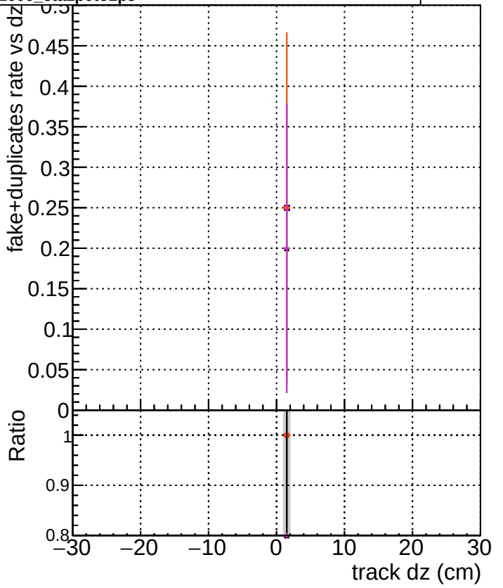
DQM original step2_pt1000_eta2p0to2p5 DQM mkFit_step2_pt1000_eta2p0to2p5 DQM angle_step2_pt1000_eta2p0to2p5 DQM fast_step2_pt1000_eta2p0to2p5 DQM pixelCPETemplate_step2_pt1000_eta2p0to2p5
