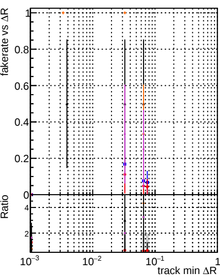
Fake rate vs \Delta R(\text{track, jet}) DQM original_step2_pt1000_eta2p0to2p5 DQM angle_step2_pt1000_eta2p0to2p5 DQM angle_step2_pt1000_eta2p0to2p5 DQM fixerCFEtemplate_step2_pt1000_eta2p0to2p5
