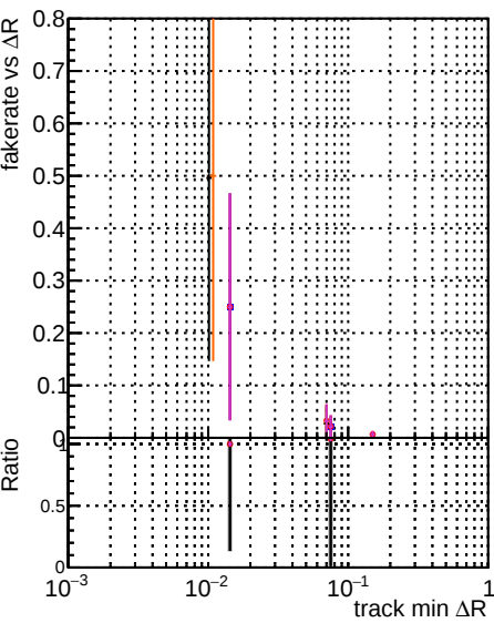
Fake rate vs \Delta R(\text{track, jet}) DQM original_step2_pt1000_eta2p0to2p5 angle_step2_pt1000_eta2p0to2p5 fixedCPETemplate_step2_pt1000_eta2p0to2p5
