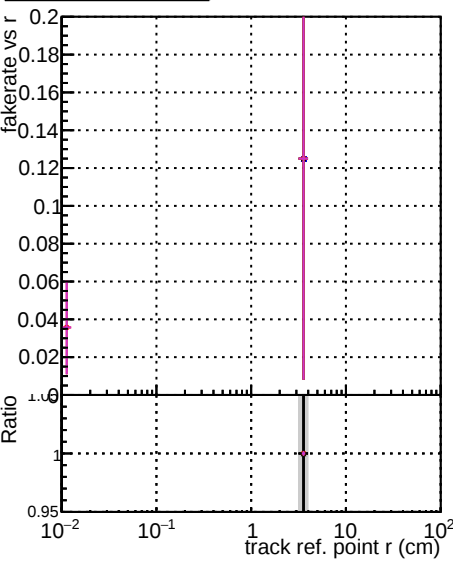
DOM original step2 pt1000 eta2p0to2p5 DOM angle step2 pt1000 eta2p0to2p5 DOM angle step2 pt1000 eta2p0to2p5 DOM fixICP template step2 pt1000 eta2p0to2p5
