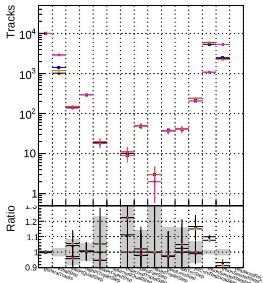
DQM original_step2_pt1000_eta1p6to2p0 mkFit_step2_pt1000_eta1p6to2p0 DQM angle_step2_pt1000_eta1p6to2p0 DQM fast_step2_pt1000_eta1p6to2p0 DQM_pixelCPE_template_step2_pt1000_eta1p6to2p0
