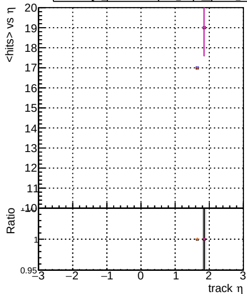
mean hit DOM original step2 pt1000 eta1p6to2p0 DOM mkrfit step2 pt1000 eta1p6to2p0 DOM angle step2 pt1000 eta1p6to2p0 DOM fast step2 pt1000 eta1p6to2p0 DOM pixelCPEtemplate step2 pt1000 eta1p6to2p0
