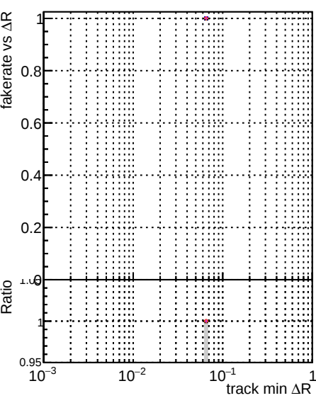
Fake rate vs \Delta R(\text{track}, \text{jet}) DQM original step2 pt1000 eta1p6to2p0 DQM original step2 pt1000 eta1p6to2p0 DQM original step2 pt1000 eta1p6to2p0 DQM original step2 pt1000 eta1p6to2p0 DQM original step2 pt1000 eta1p6to2p0
