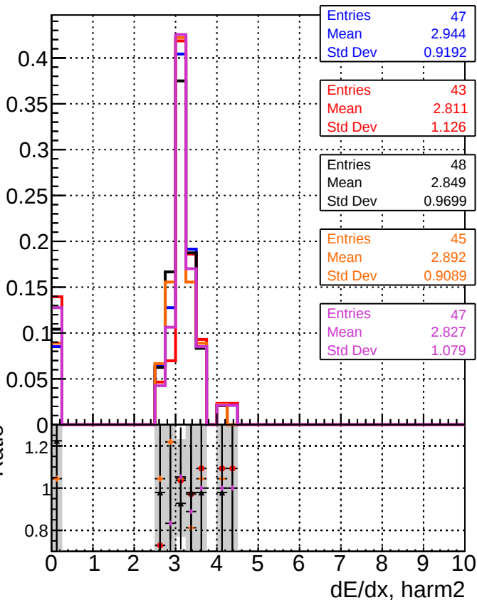
DQM_original_step2_pt1000_eta1p6to2p0 DQM_mkFit_step2_pt1000_eta1p6to2p0 DQM_angle_step2_pt1000_eta1p6to2p0 DQM_fast_step2_pt1000_eta1p6to2p0 DQM_pixelCPETemplate_step2_pt1000_eta1p6to2p0
