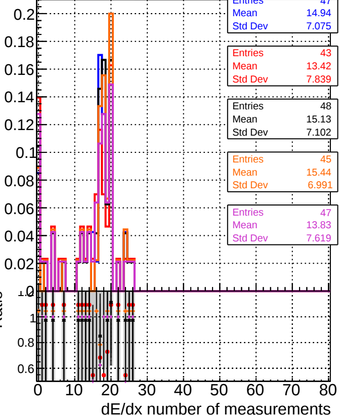
DQM_original_step2_pt1000_eta1p6to2p0 DQM_mkFit_step2_pt1000_eta1p6to2p0 DQM_angle_step2_pt1000_eta1p6to2p0 DQM_fast_step2_pt1000_eta1p6to2p0 DQM_pixelCPETemplate_step2_pt1000_eta1p6to2p0
