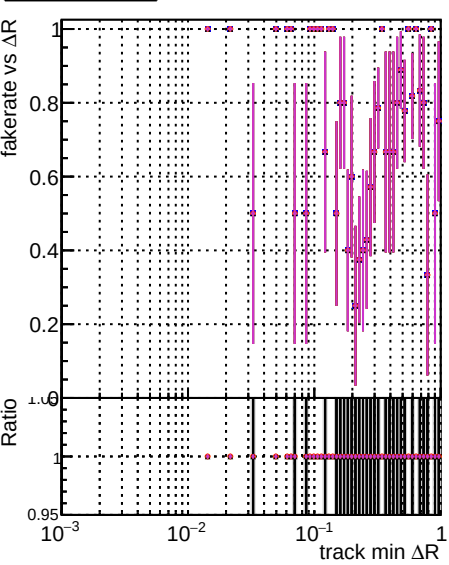
Fake rate vs ΔR(track, jet) Legend: original_step2_pt1000_eta1p0to1p4 angle_step2_pt1000_eta1p0to1p4 fixICP_template_step2_pt1000_eta1p0to1p4
