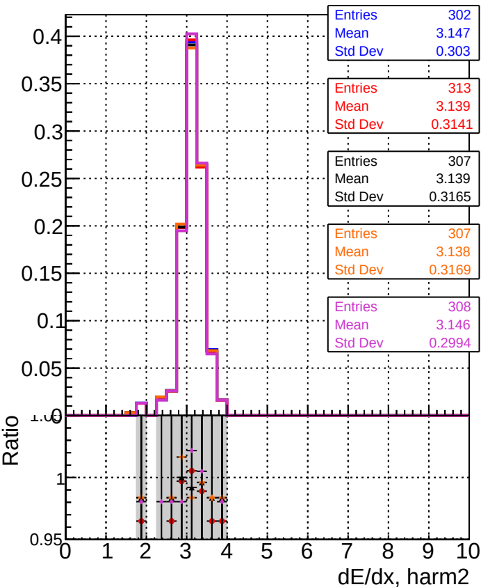
DQM original step2 pt1000 eta1p0to1p4 DQM mkFit step2 pt1000 eta1p0to1p4 DQM angle step2 pt1000 eta1p0to1p4 DQM fast step2 pt1000 eta1p0to1p4 DQM pixelCPETemplate step2 pt1000 eta1p0to1p4
