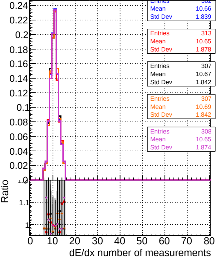
DQM original step2 pt1000 eta1p0to1p4 DQM mkFit step2 pt1000 eta1p0to1p4 DQM angle step2 pt1000 eta1p0to1p4 DQM fast step2 pt1000 eta1p0to1p4 DQM pixelCPETemplate step2 pt1000 eta1p0to1p4
