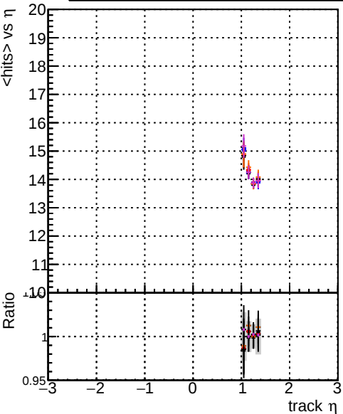
mean hits vs \eta DOM original step2 pt1000 eta1p0to1p4 DOM mkrfit_step2 pt1000 eta1p0to1p4 DOM angle_step2 pt1000 eta1p0to1p4 DOM fast_step2 pt1000 eta1p0to1p4 DOM pixelCPEtemplate_step2 pt1000 eta1p0to1p4
