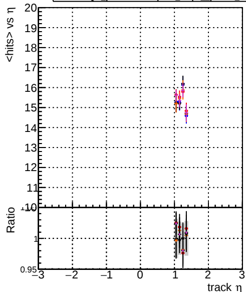
mean hit DOM original_step2_pt1000_eta1p0to1p4 DOM mkrfit_step2_pt1000_eta1p0to1p4 DOM angle_step2_pt1000_eta1p0to1p4 DOM fast_step2_pt1000_eta1p0to1p4 DOM pixelCPEtemplate_step2_pt1000_eta1p0to1p4
